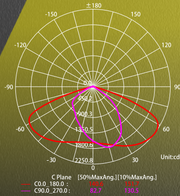
C plane lighting distributions
